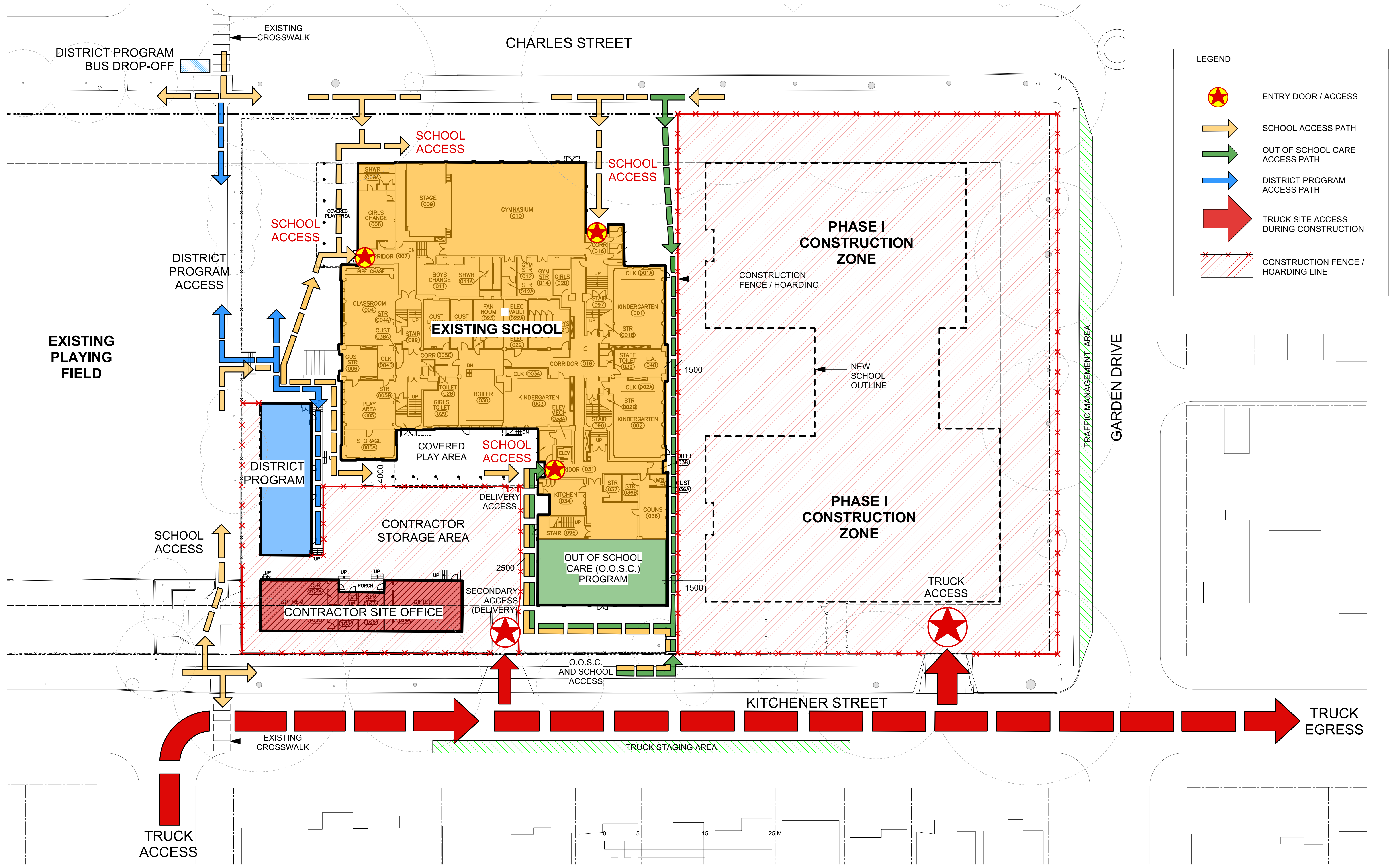
1 LORD NELSON SCHOOL ACCESS DIAGRAM DURING PHASE I CONSTRUCTION Scale: 1:250
